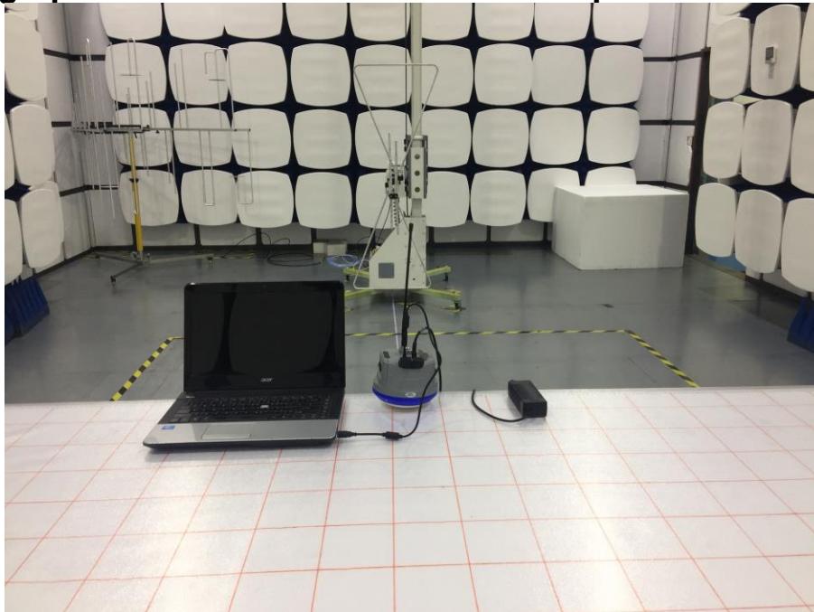
Photograph – Radiated Emission Test Setup-Below 1GHz
